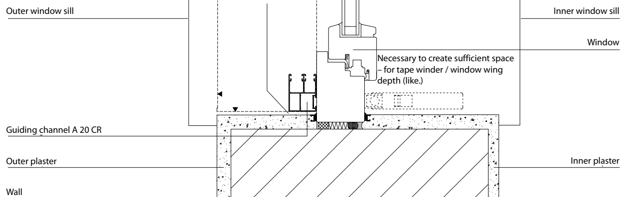
Detailed connection – side view (lower part)
