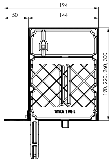
Cross-section of revealed VIVA box + P 020/05, P 080/05, P 081/05 190 x 140b 220 x 140b 260 x 140b 300 x 140b
