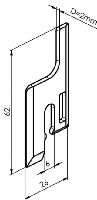
Spacing pad P 640 2-02670-XXXX-0
