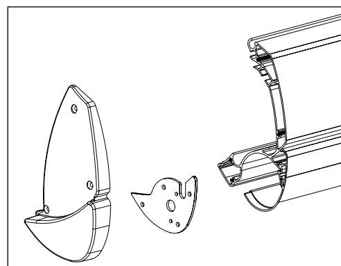
Extension pole variovalance
