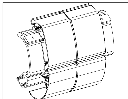
Coupling variovalance
