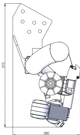
Console for roofing – cross arms
