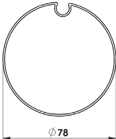
Winding roller (6-011084)
