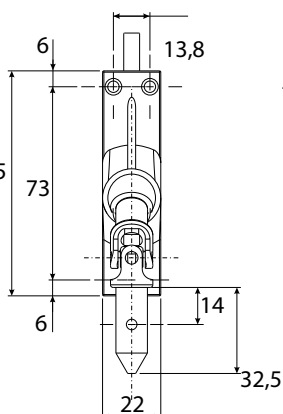
cardan joint 45°
