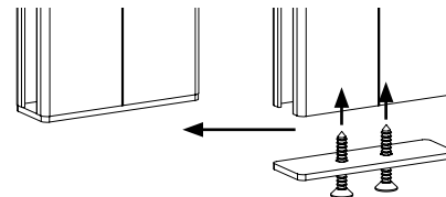
End stop pin guide assembly intermediate guide
