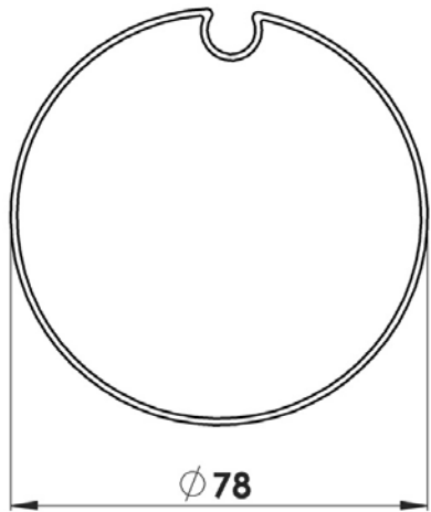
Winding roller (6-011084)
