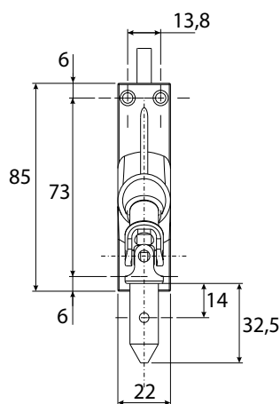
cardan joint 45°
