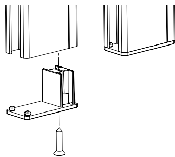
End stop
